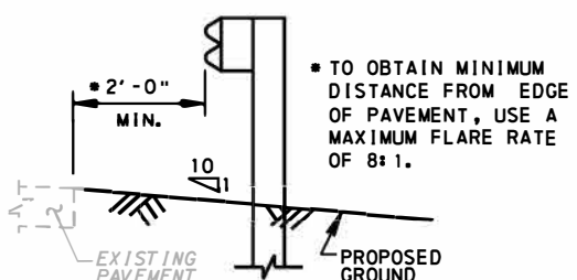
APPROACH GUIDE RAIL DETAIL ALL GUIDE RAIL APPROACH SECTIONS N. T. S.
